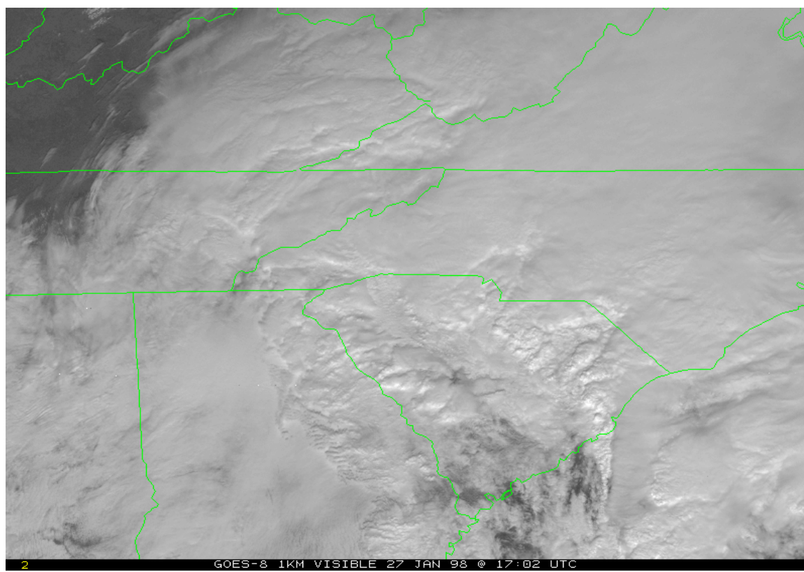
Figure 6. GOES-8 1KM Visible Image, 27 Jan 98 at 17:02 Z
