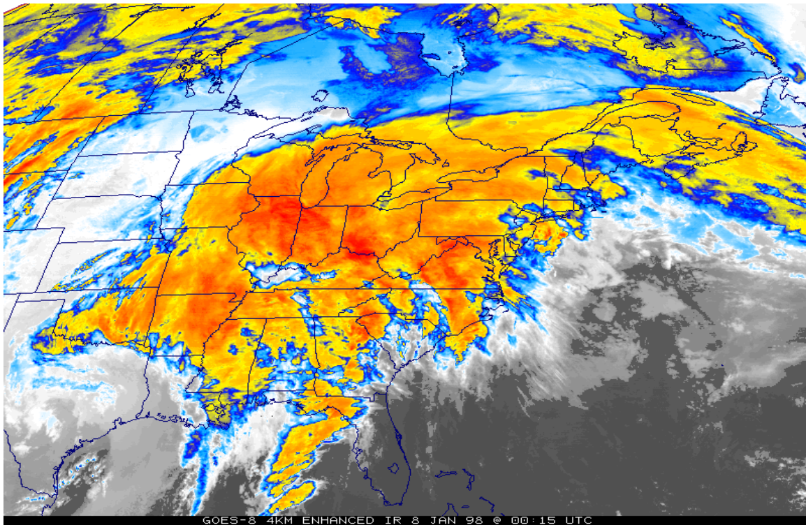
Figure 3. GOES- 8 Infrared Image, 08 Jan 98 at 00:15 Z
