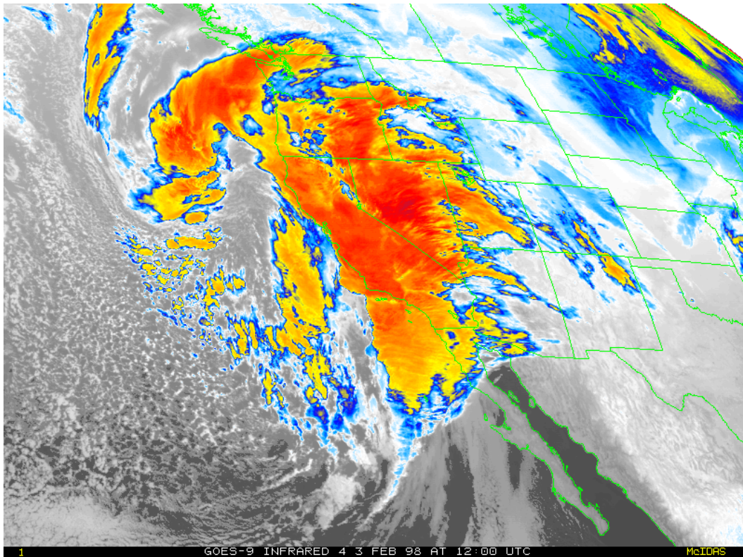
Figure 7. GOES-9 Infrared Image, 3 Feb 98 at 12:00Z
