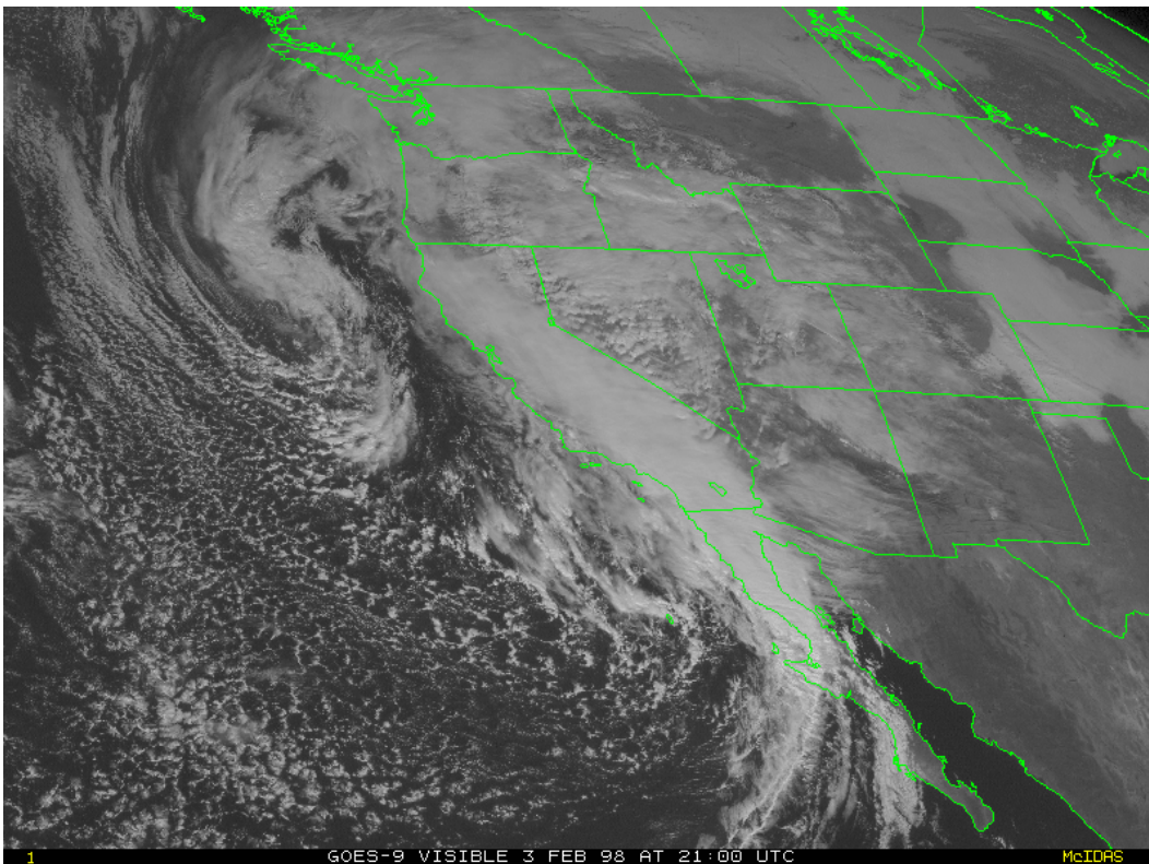
Figure 8. GOES-9 Visible Image, 3 Feb 98 at 21:00Z
