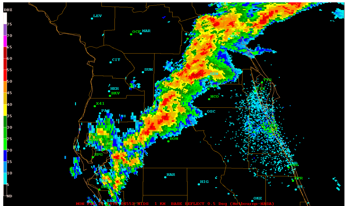
Figure 10. NEXRAD Radar Reflectivity 23 Feb 98 at 04:55Z
