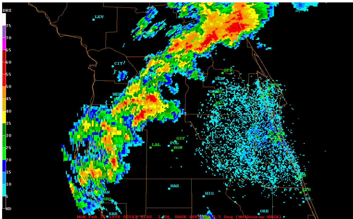
Figure 9. NEXRAD Radar Reflectivity 23 Feb 98 at 03:56Z
