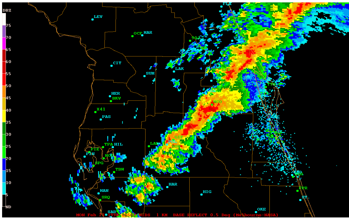
Figure 11. NEXRAD Radar Reflectivity 23 Feb 98 at 05:50Z
