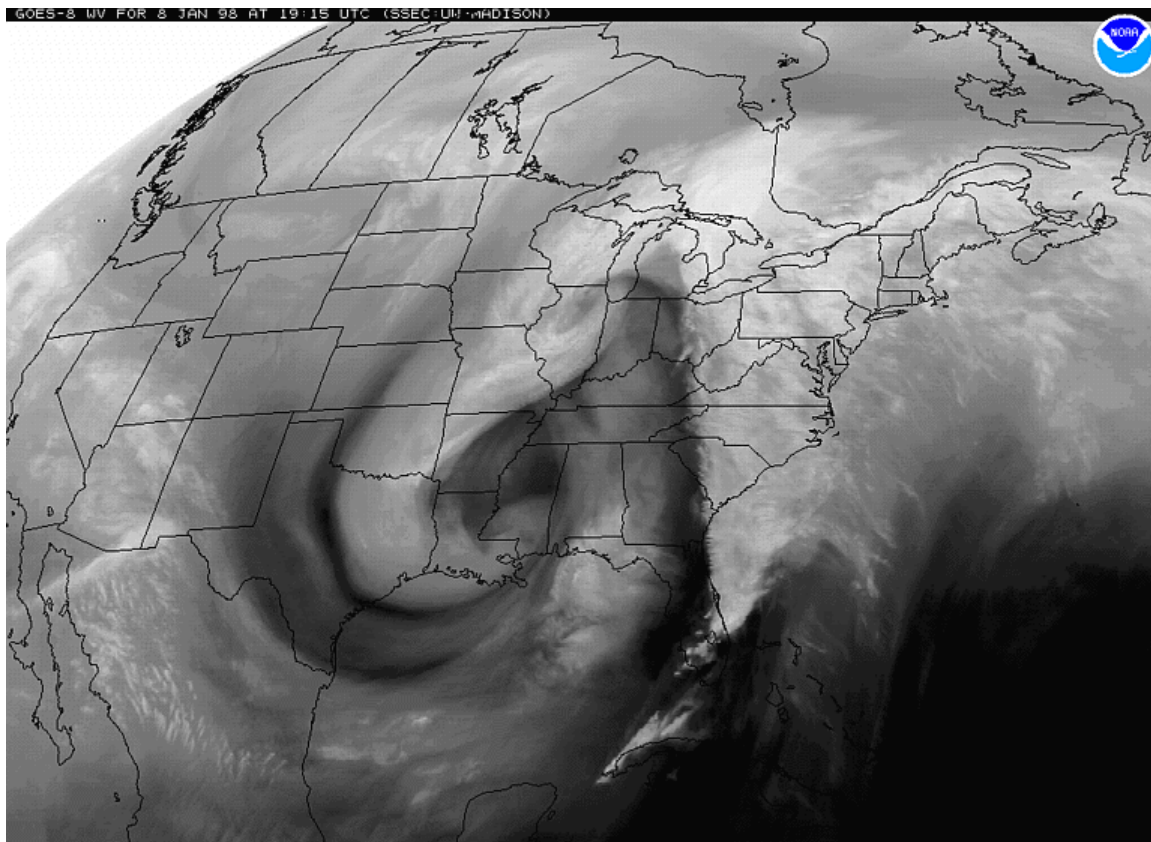
Figure 5. GOES-8 Water Vapor Image, 08 Jan 98 at 19:15Z
